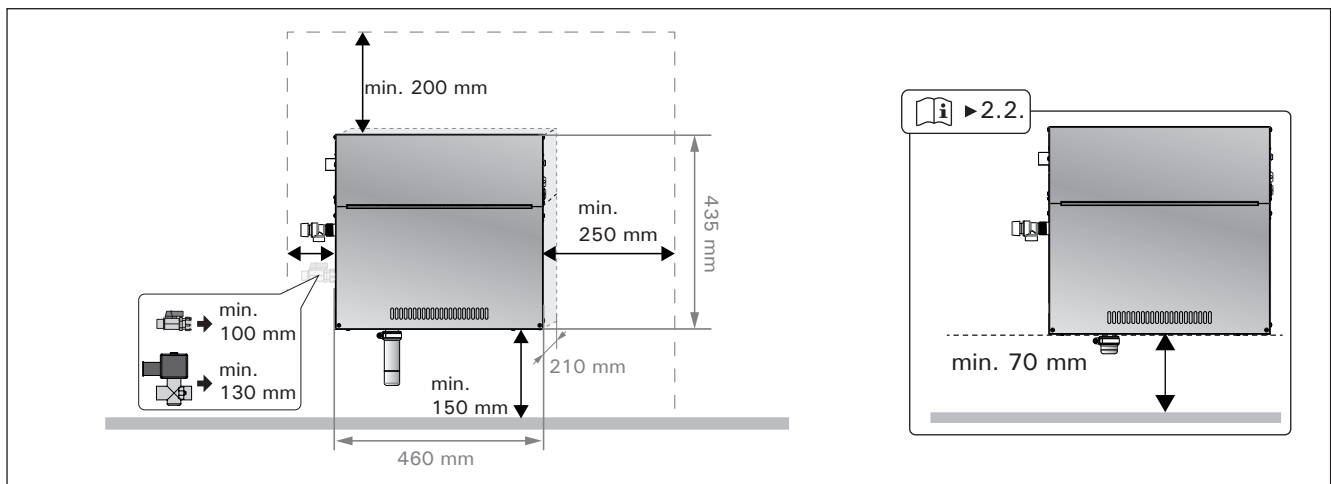
Figure 4. Installation measurements
